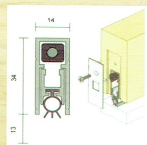
RP8 Acoustic Door Seal
